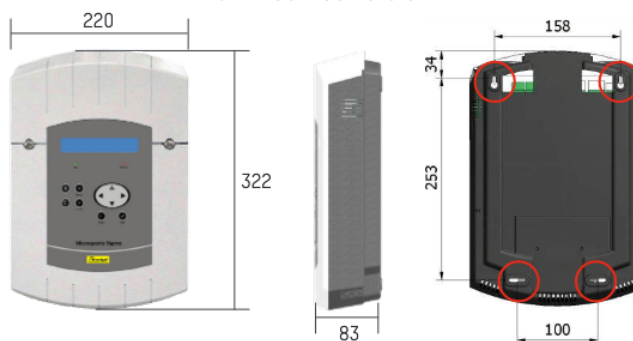
Wall-mounted version
